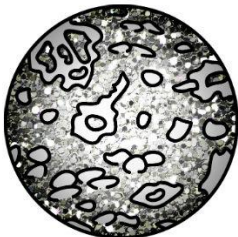
Mercury
