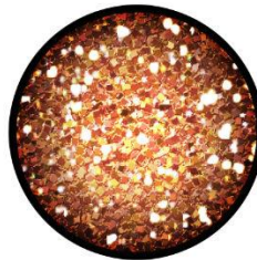
Dwarf Planet
